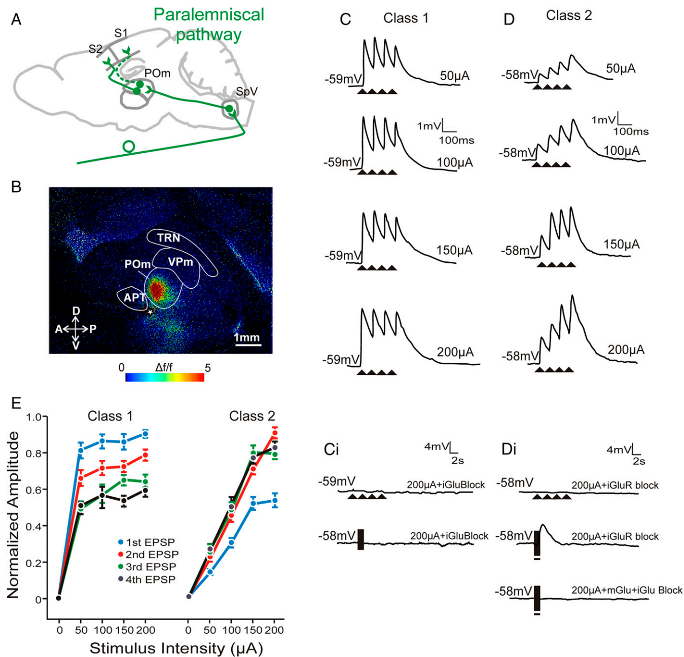
Fig. 2. Electrical stimulation of the paralemnisal pathway shows both class 1 and 2 properties in POM synapses. (A) Schematic of the paralemnisal pathway from brainstem SpV to S1 and S2 via POM. (B) FA image showing selective activation of POM to electrical stimulation of fibers in the paralemnisal pathway from brainstem (white star, 50 \mu A). (C) Example EPSP traces of a POM cell in response to 10 Hz electrical stimulation at increasing intensities. Paired-pulse depression is observed, a class 1 property. (C, i ) Traces from the same cell during high-intensity stimulation at 10 Hz (upper trace) and high-frequency stimulation (lower trace) in the presence of ionotropic glutamate receptor blockers. (D) Example EPSP traces of a POM cell in response to 10 Hz stimulation with paired-pulse facilitation, a class 2 property. (D, i ) Traces from the same cell during high-intensity stimulation at 10 Hz (upper trace) and high-frequency stimulation (middle trace) in the presence of ionotropic glutamate receptor blockers. Note the prolonged membrane depolarization during high-frequency stimulation (middle trace) could be abolished by metabotropic receptor antagonists (bottom trace). (E) Normalized EPSP response amplitudes as stimulation intensity increases for both classes. EPSPs were normalized to the EPSP amplitude that was the highest response at any stimulation intensity within each class. In contrast to cells showing a class 1 response ( n = 11 ), class 2 cells ( n = 28 ) showed EPSP amplitudes that increased dependent on stimulation intensity. Error bars represent mean \pm SEM. APT, anterior pretectal nucleus; POM, posterior medial nucleus; SpV, spinal trigeminal nucleus; TRN, thalamic reticular nucleus; VPm, ventral posterior medial nucleus.
