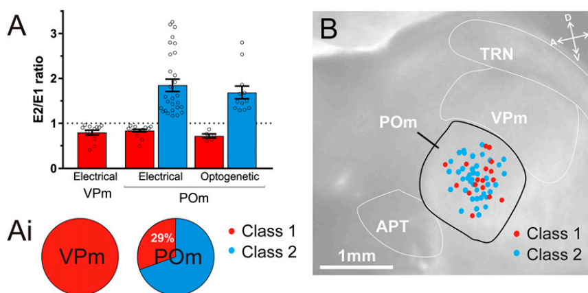
Fig. 4. Summary of class 1 and class 2 responses to lemniscal and paralemniscal inputs to VPm and POM using electrical and optogenetic stimulation. (A) The E2/E1 ratios (second pulse amplitude/first pulse amplitude) of all recorded cells in response to 10 Hz stimulation of the lemniscal pathway to VPm ( n = 12 , tested electrically) and the paralemniscal pathway to POM ( n = 39 tested electrically and n = 17 optogenetically). Paired-pulse depression (E2/E1 ratio < 1 ) indicates a synapse has class 1 properties (red bars), and paired-pulse facilitation (ratio > 1 ) indicates a synapse has class 2 properties (blue bars). Note the consistency of ratios for each class across nuclei and stimulation technique. (A, i) Proportions of class 1 and class 2 cells in VPm ( n = 12 ) and POM ( n = 56 ). In the case of POM, these proportions represent the combination of electrical and optogenetic experiments. (B) Locations of recorded POM cells classified as class 1 and class 2. Locations were reconstructed from photos taken during electrical and optogenetic stimulation recordings and superimposed on a representative image of the paralemniscal slice. The positions of cells classified as class 1 (red dots, n = 16 ) and class 2 (blue dots, n = 40 ) did not show obvious location trends. Error bars represent mean \pm SEM. APT, anterior pretectal nucleus; POM, posterior medial nucleus; TRN, thalamic reticular nucleus; VPm, ventral posterior medial nucleus.
